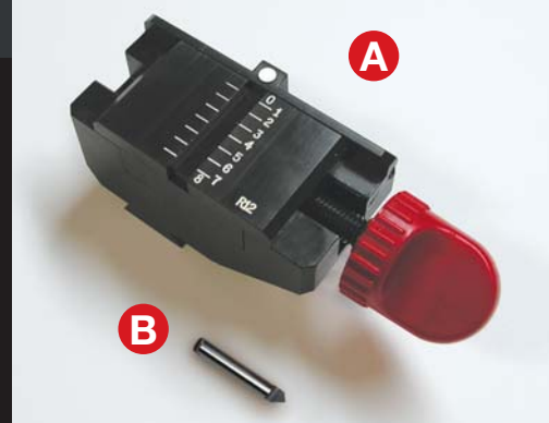
A. Single Jaw - R12 (code D733984ZB) B. Cutter - W146 (code D734267ZB)
