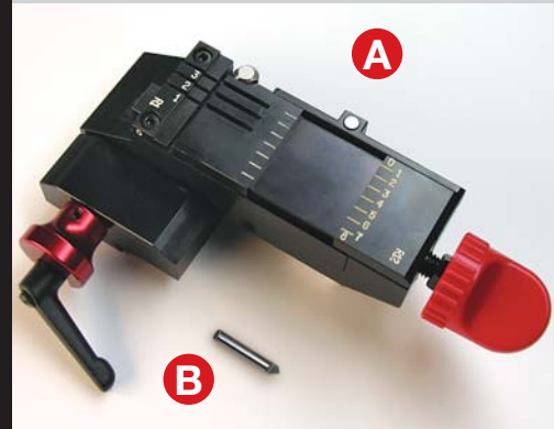
A. Double Jaw - R1/R12 (code D734232ZB) B. Cutter - W146 (code D734267ZB)
